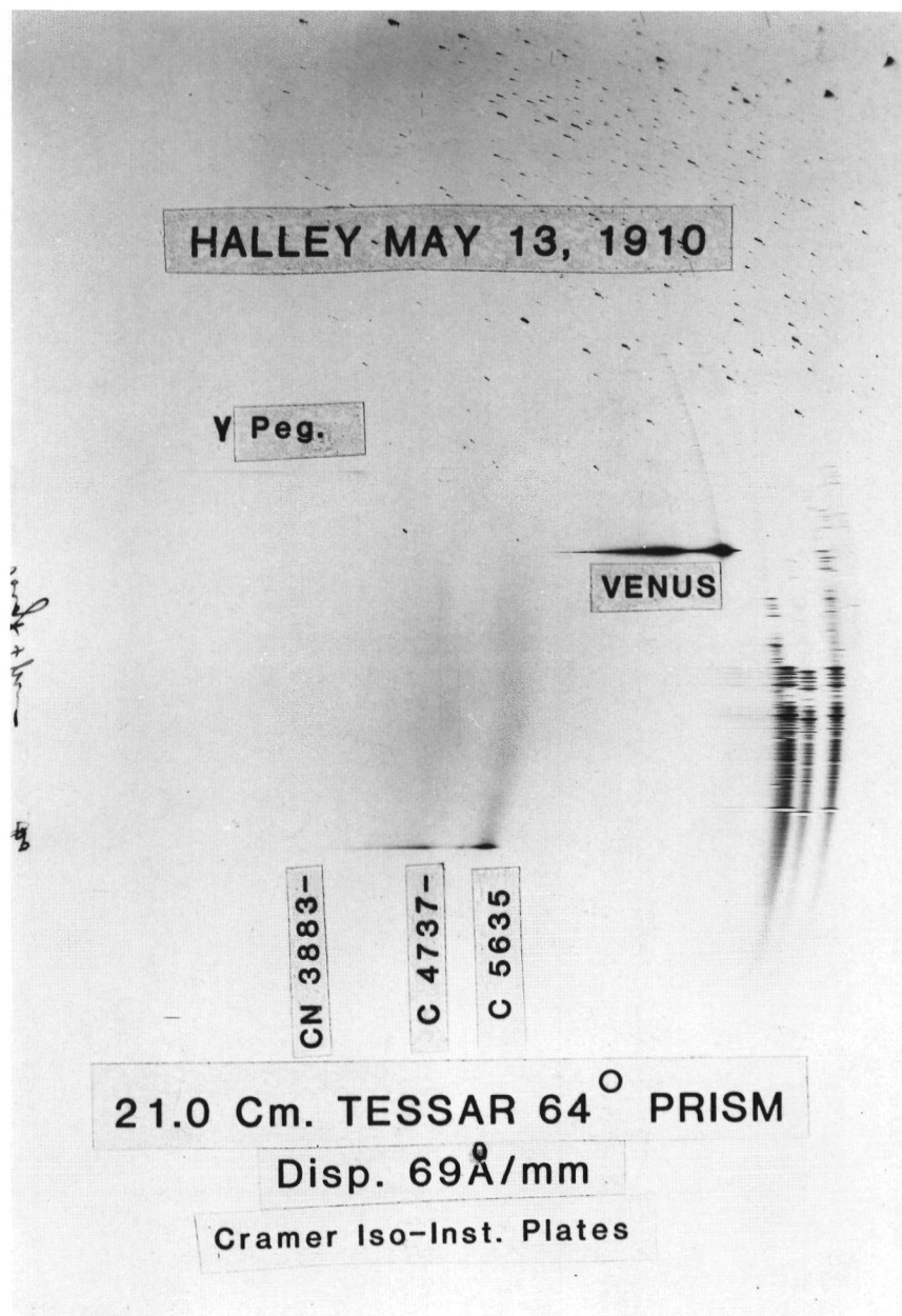
Figure 8. Objective prism spectrogram of Comet Halley obtained on May 13, 1910.
